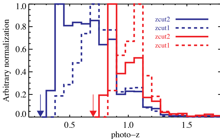
Figure 5. Redshift distribution of background galaxies selected using the ZCUT1 (dashed lines) and ZCUT2 (solid lines) criterion for the lowest (blue lines) and highest (red lines) redshift clusters in the S/N > 5 . The arrow indicates the redshift of the foreground cluster. The redshift distributions for ZCUT2 and ZCUT1 are significantly different, but their relative weak-lensing signals are not.
