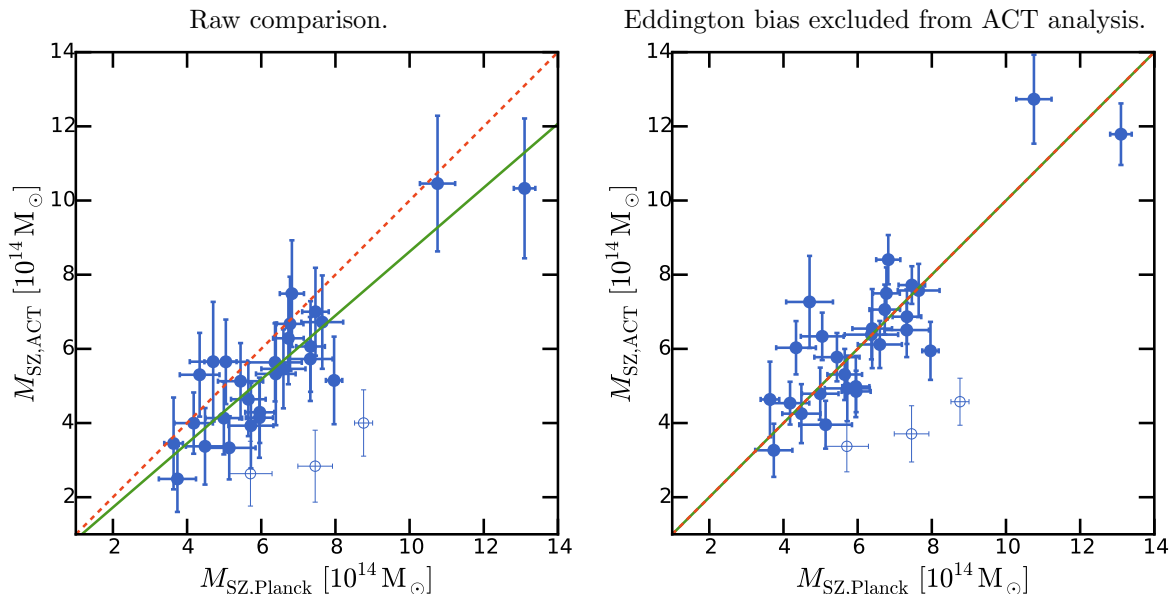
Figure 6. Comparisons between the inferred tSZ masses from ACT and Planck for the same 31 clusters. The open circles are clusters that we exclude from this analysis (see section 6 for more details). Left: shows the comparison of the published masses for both experiments. Right: shows the comparison when we reanalyze the ACT clusters without accounting for Eddington bias. The best fit slopes are shown with the green solid lines and slopes of unity are shown by the red dashed lines. The raw comparison has a systematic difference between ACT and Planck of 16%. The reanalysis shows that we can remove this systematic offset between ACT and Planck masses by not accounting for the Eddington bias in the ACT analysis and get a slope of 1.00 \pm 0.03 . We conclude from this figure and the contents of both the Planck SZ source papers [15, 16] and the Planck 2015 Release Explanatory Supplement that the Eddington bias was not included in the published Planck SZ masses.
