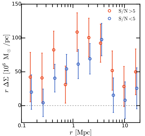
Figure 2. Stacked weak-lensing measurements ( \Delta\Sigma ) of the S/N > 5 (red circles) and S/N < 5 (blue circles) clusters from the tSZ selected ACT equatorial sample. The thick error bars are the statistical errors and these errors are uncorrelated because they are shape noise dominated. Note that we offset the data on the x-axis for clarity and show r \Delta\Sigma to reduce the dynamic range of the y-axis.
