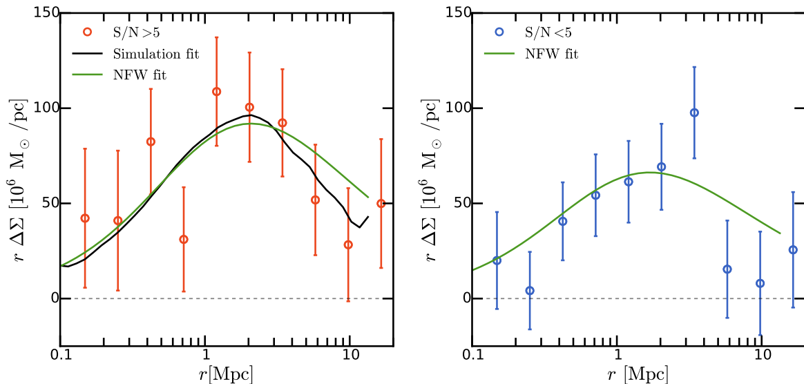
Figure 3. Comparison of the best fit models to the weak-lensing measurements ( \Delta\Sigma ), where mass is the free parameter in the fit. Left: the weighted \Delta\Sigma of the S/N > 5 sample with the best fit models from simulations (black lines) and NFW profile (green lines). Right: the weighted \Delta\Sigma of the S/N < 5 sample with the best fit NFW profiles (green line). The error bars show the statistical uncertainties. Note that we show r\Delta\Sigma to reduce the dynamic range of the y-axis.
