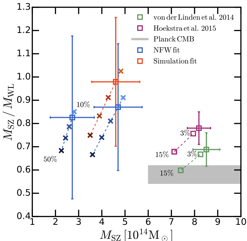
Figure 7. Comparison between the ratio of the tSZ masses ( M_{\text{SZ}} ) to weak-lensing masses ( M_{\text{WL}} ) as a function of M_{\text{SZ}} . The CS82 weak-lensing masses of ACT clusters are shown by the red and blue squares for the simulation and NFW fit, respectively. The light to dark crosses show the degeneracy locus for the assumption on scatter in the Y-M relation from 10% (lightest) to 50% (darkest), the fiducial assumption is 20% represented by the squares. Previous weak-lensing calibrations of Planck clusters are shown by the open squares at the mean M_{\text{SZ}} mass of the sample, the green squares for [37] and the purple squares for [36]. The squares without a percentage label show the original measurements and the squares connected by the dashed lines show the 3-15% range for the Eddington corrected measurements. The 1 - b expected by the Planck primary CMB results is represented by the gray band. The weak-lensing mass calibration of ACT tSZ masses are consistent with previous calibrations of Planck tSZ masses [e.g., 36, 37]. The Eddington bias corrections to the Planck tSZ masses bring the measured 1 - b factors from [37] and [36] consistent with or closer to the inferred 1 - b by fixing the cosmological parameters to the Planck primary CMB results.
