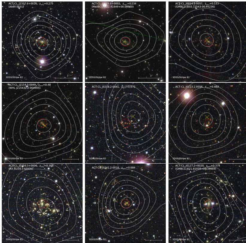
Figure 1. Gallery of ACT clusters in the CS82 footprint with a S/N > 5 ordered left to right and top to bottom in descending S/N . The imaging is from the Stripe 82 SDSS co-add ( g , r , and i band). White contours and yellow crosses show the tSZ contours and peak, respectively. The position of the BCG is circled in red, which is used as the centroid for the weak-lensing measurements.
