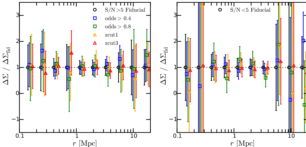
Figure 4. Ratio of weak-lensing signals for the fiducial photometric redshift (photo- z ) cuts of ZCUT2 and ODDS > 0.5 (black circles) to other photo- z cuts. Changing the cuts on the photo- z s does not have a significant effect on the weak-lensing results. Making stricter cuts and removing more background galaxies does increase the statistical uncertainties. We offset the data on the x-axis for clarity.
